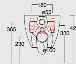
Cod. 45000101 Vaso sospeso Wunder Wunder WC wall hung
